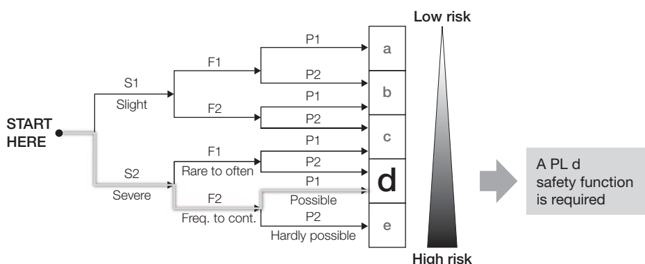
Figure 3-5 Example of PL risk graph
