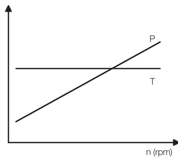
Figure 6.1 Typical torque and power curves in a constant torque application.
