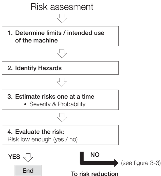
Figure 3-2 Risk assessment and evaluation according to EN ISO 14121-1
