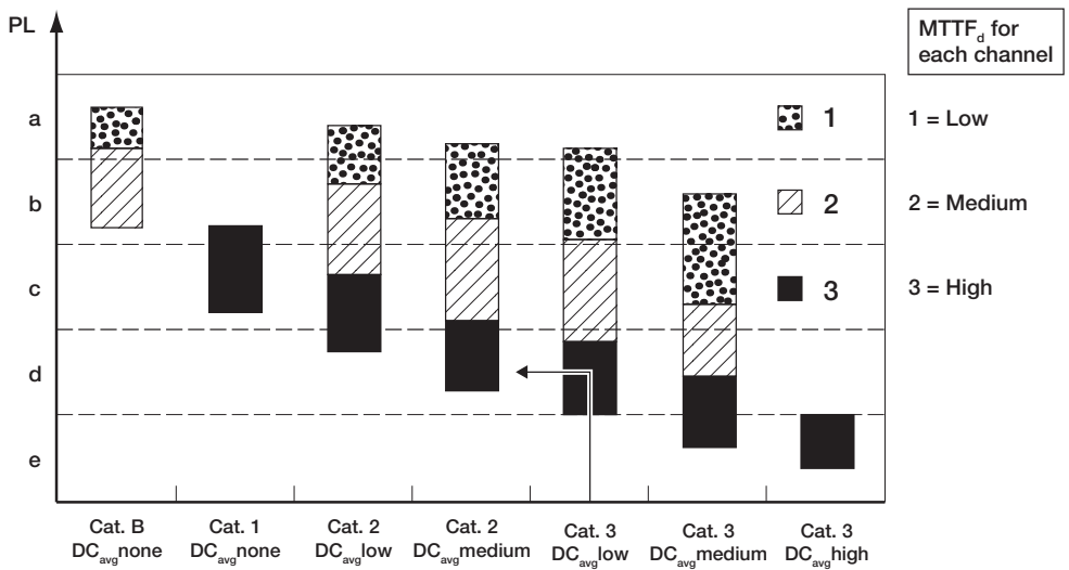
Figure 3-8 Example verification of PL
