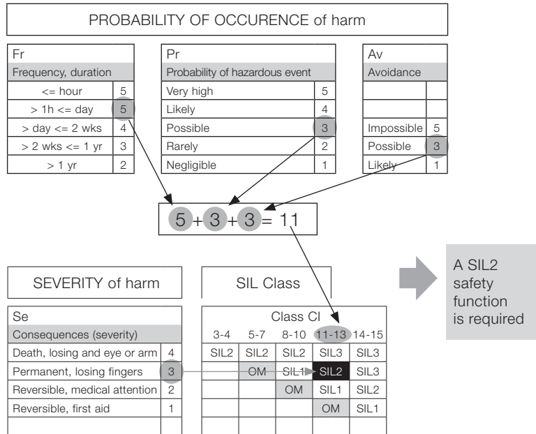
Figure 3-4 Example of SIL assignment table
