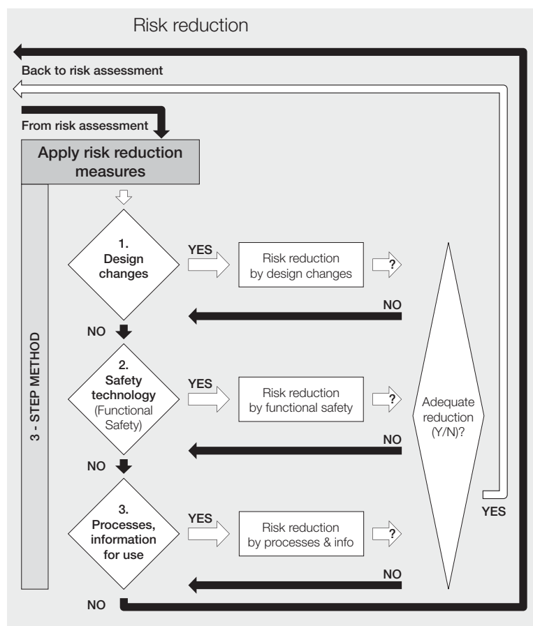
Figure 3-3 The 3-step method for risk reduction according to EN ISO 12100-1
