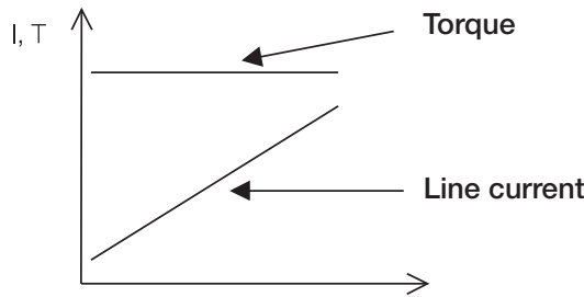
Figure 9.1 Line current in a constant torque application. Line current is small at low speed.
